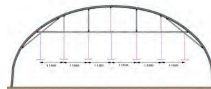
9.30 m tunnel: up to 7 crop lines
